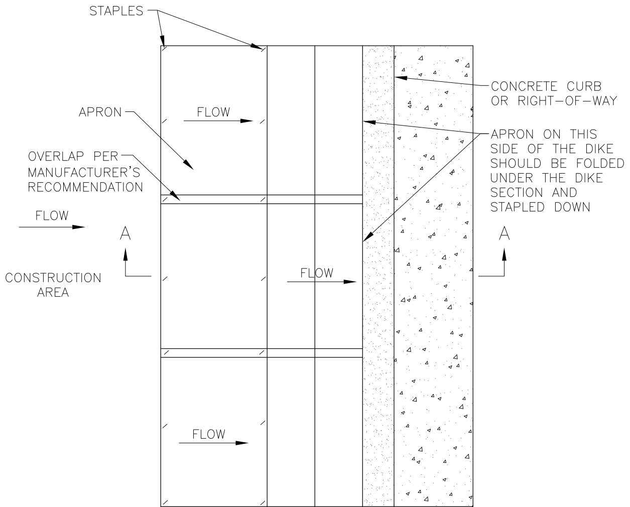
DIKE PLAN VIEW
