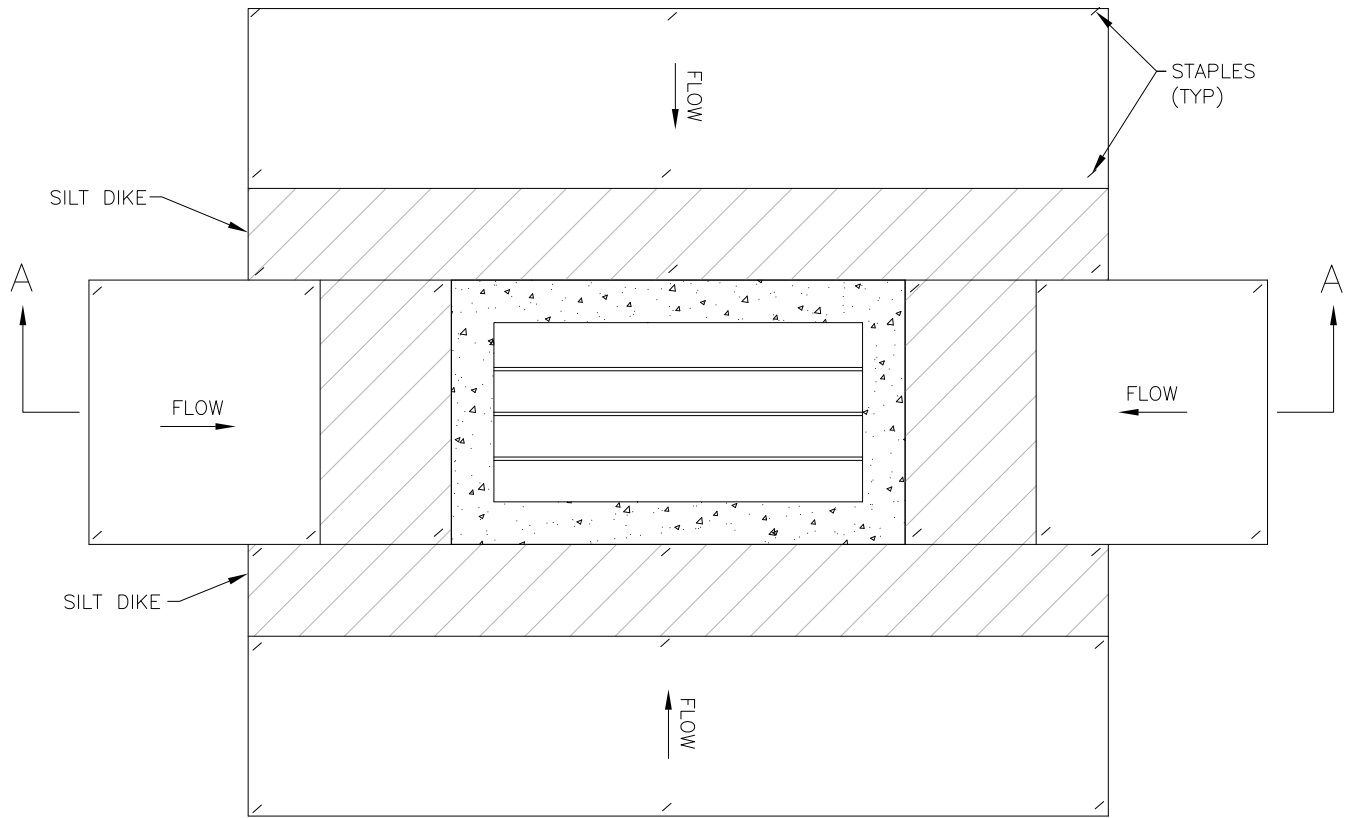
DROP INLET PLAN VIEW
