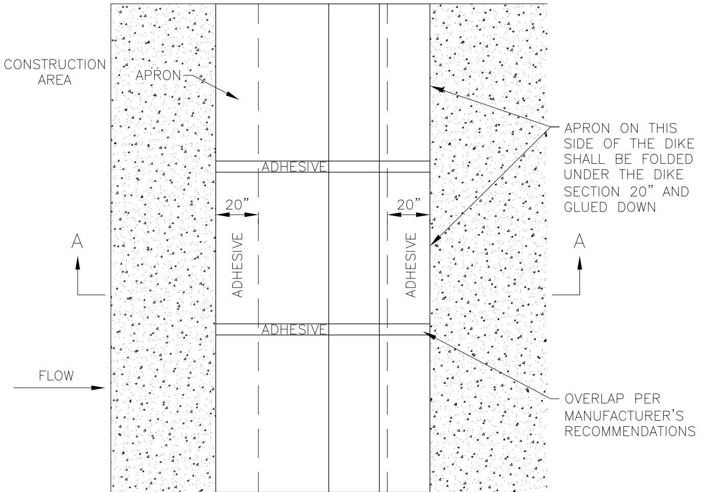
DIKE PLAN VIEW
