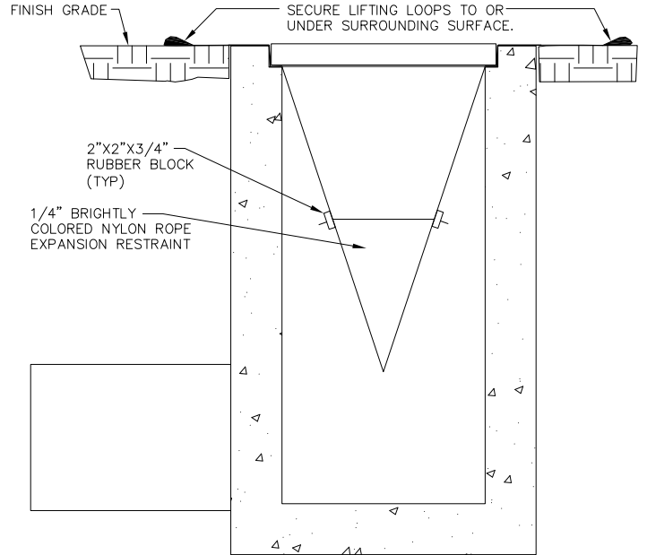
ELEVATION VIEW PROFILE VIEW OF INSTALLED FILTER SACK
