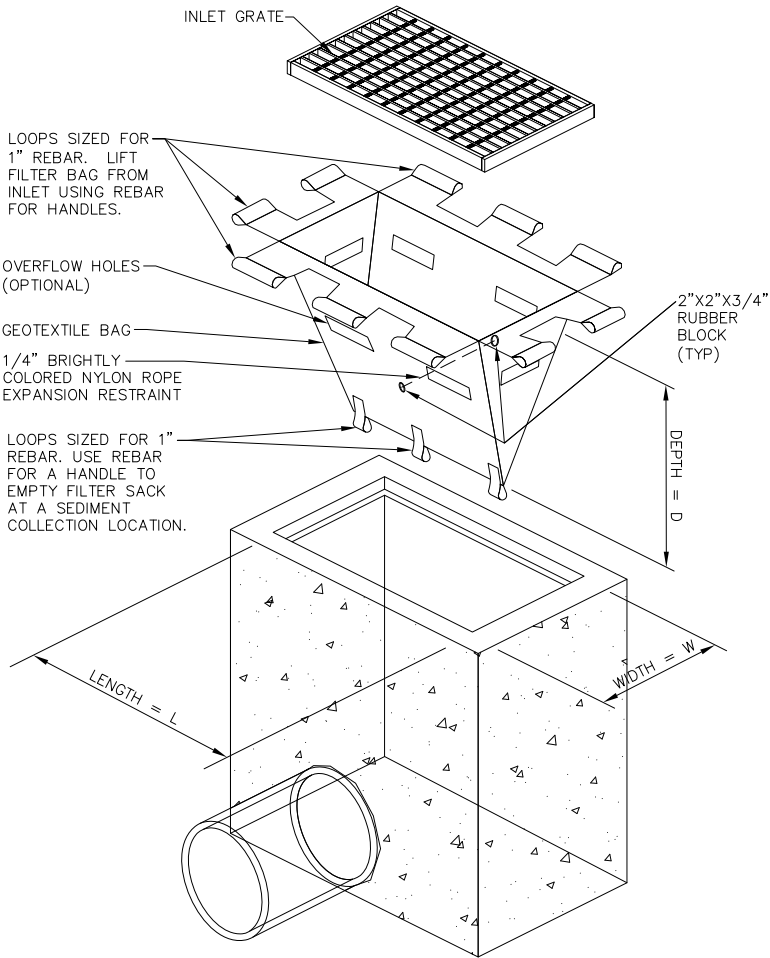
ISOMETRIC VIEW
