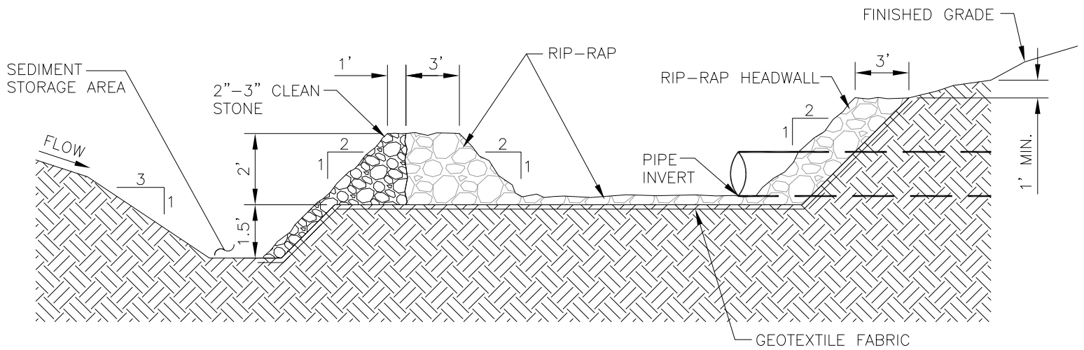
CROSS-SECTION
