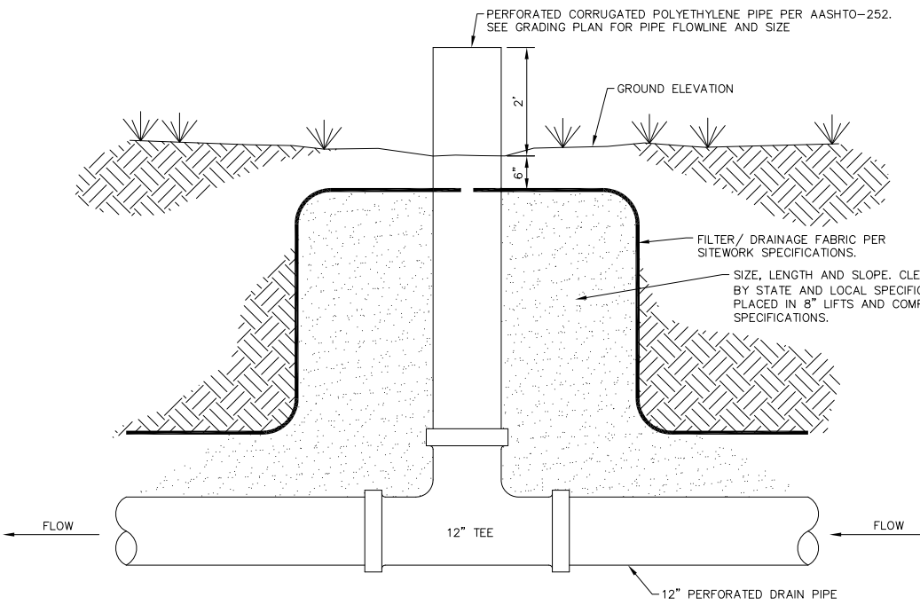
RISER PIPE DETAIL NO SCALE
