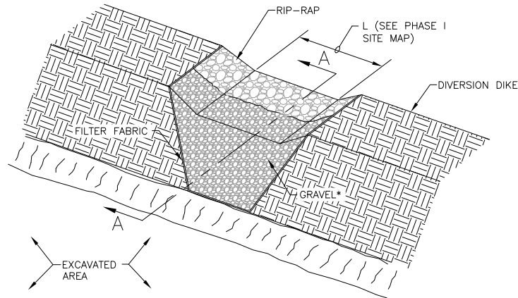
OUTLET (PERSPECTIVE)
