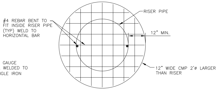
ROUND TRASH RACK
