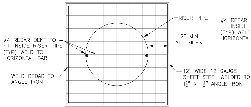
SQUARE TRASH RACK
