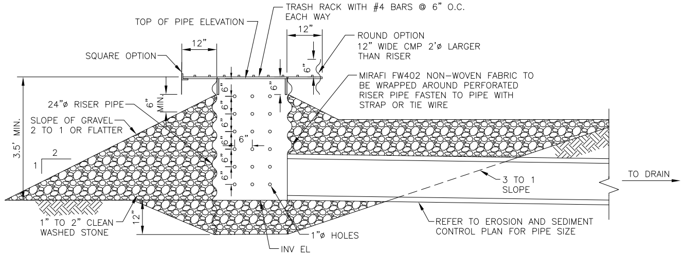
SQUARE TRASH RACK
