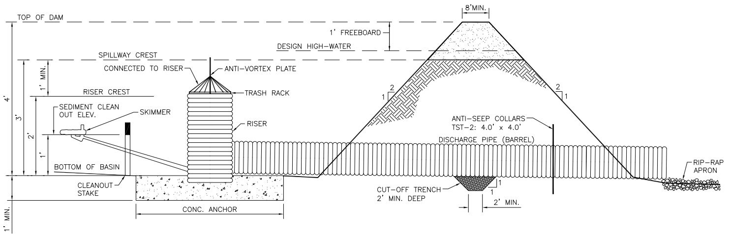
SECTION A-A THROUGH EMBANKMENT
