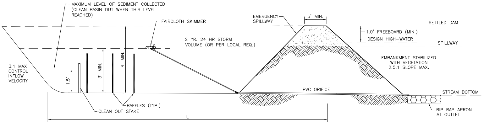
SECTION A-A THROUGH EMBANKMENT
