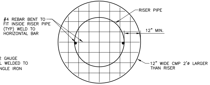
ROUND TRASH RACK
