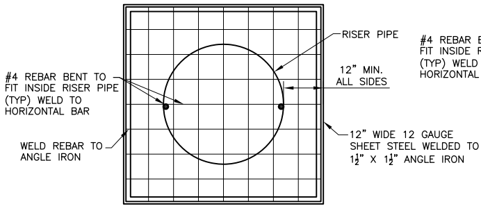
SQUARE TRASH RACK
